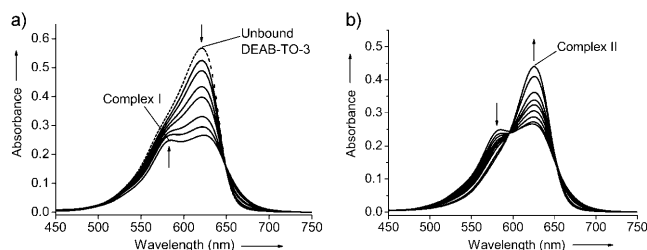
Figure 2. Absorption spectra during the titration of a 5 \mu\text{M} solution of DEAB-TO-3 with CT DNA at 20 ^{\circ}\text{C} in buffer. The [base pair]/[DEAB-TO-3] molar ratios are 0.33, 0.63, 1.25, 1.67, 2.5, 3.3, and 5 in (a) and 6.5, 8, 10, 12.5, 15, 20, 30, 45, and 60 in (b). The black dashed line refers to DEAB-TO-3 without CT DNA. The arrows indicate how the absorbance bands respond to the increases in the CT DNA concentration.
